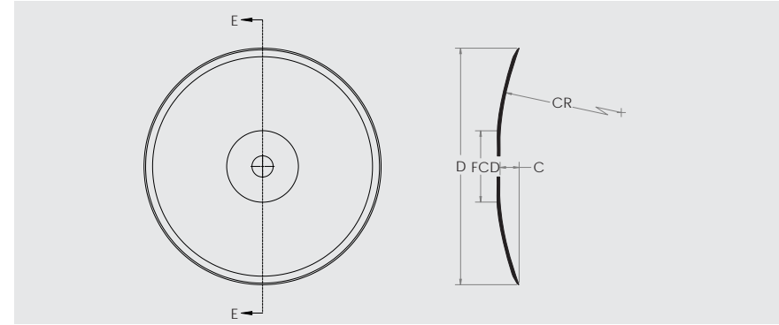
Plain & Notched Flat Center Disc Dimensions
