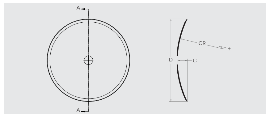
Rollable Boron Disc Blades - Plain
